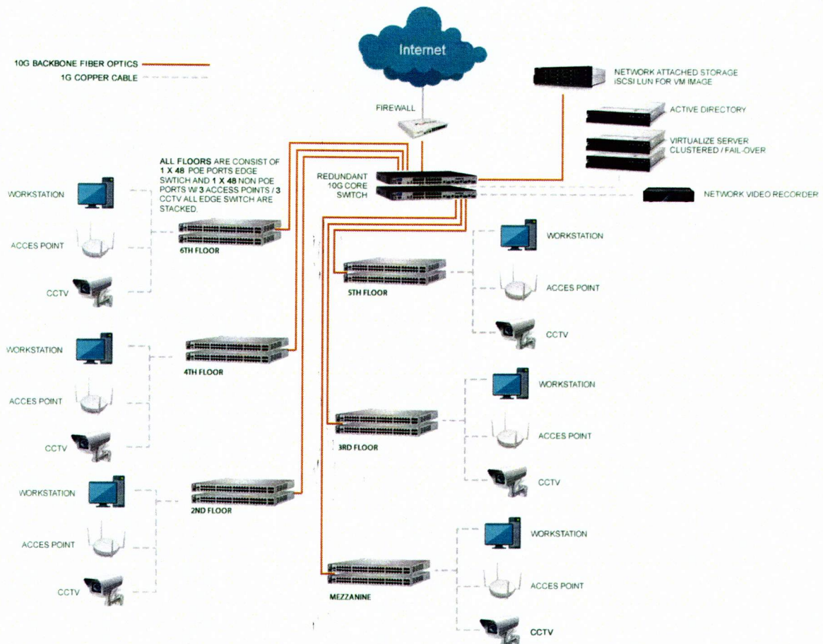
Figure 1. SHFC Network Infrastructure Layout
